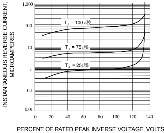
Fig. 3-TYPICAL REVERSE CHARACTERISTICS
